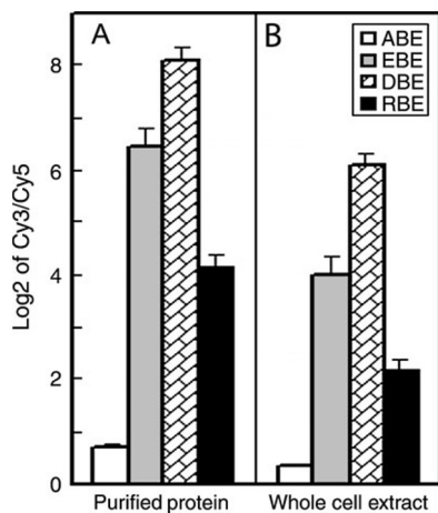
Figure 2. Relative DNA-Binding Affinity of GST-TINY2 Purified from Two Different Hosts.
