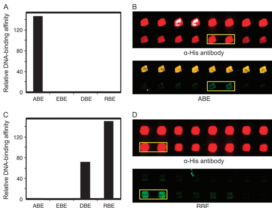
Figure 3. DNA-Binding Affinity and Specificity of ANT and RAV1.
