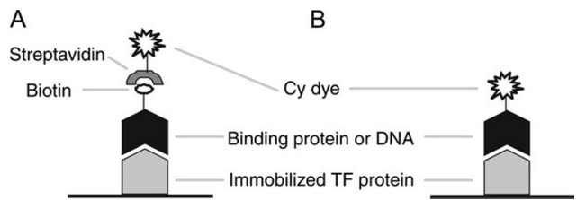
Figure 10. Strategies for Detecting Protein–DNA and Protein–Protein Interactions.
