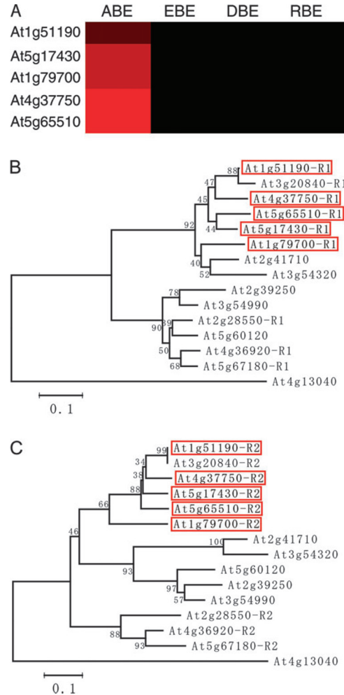
Figure 6. DNA-Binding and Phylogenetic Analysis of AP2 Subfamily Members.
