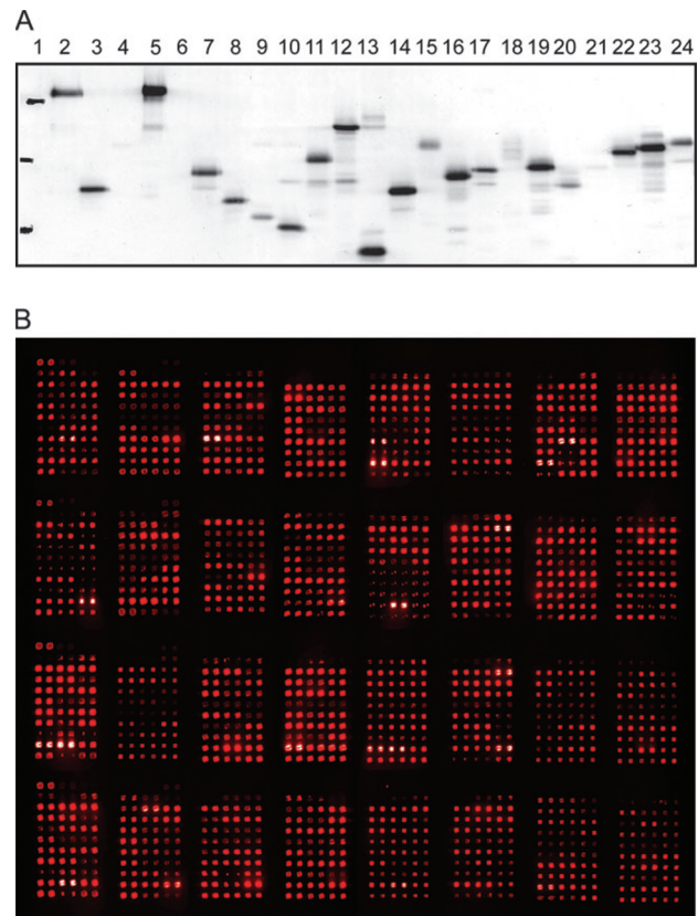
Figure 1. Construction of Arabidopsis TF Protein Microarrays.
