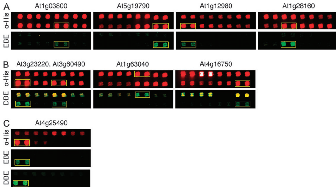
Figure 4. Examples of Protein–DNA Binding Assays on Protein Microarrays.
