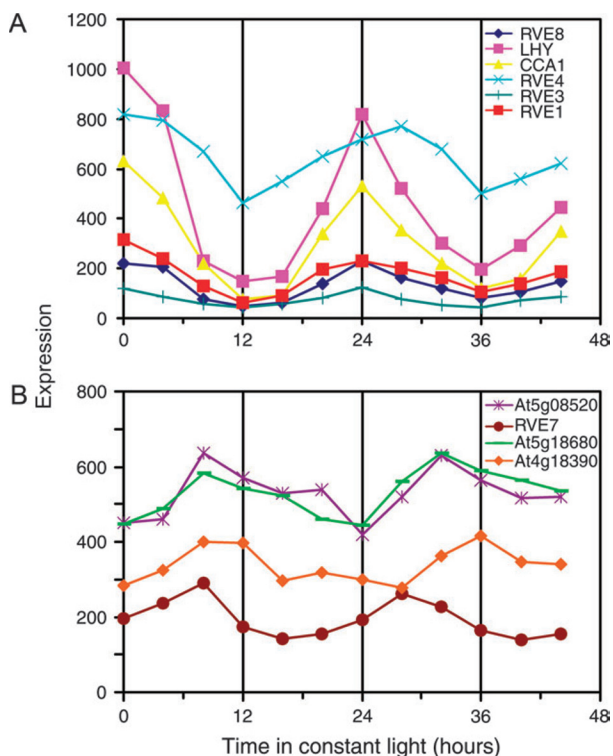
Figure 7. Transcription Patterns of 10 EE-Binding Myb TFs under Constant Light.
